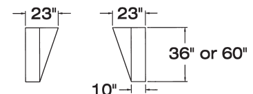
Mounting Legs
