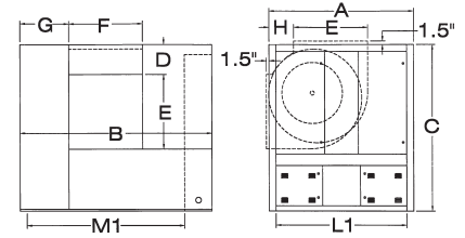
Base Heater
